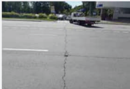
Transverse crack
